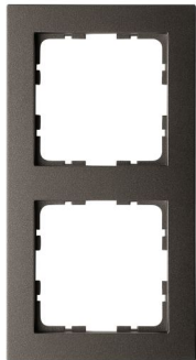
G1002Z 2-gang W 80mm H 151mm D 9mm
