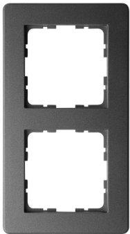
G1102B 2-gang W 86mm H 157mm D 9mm
