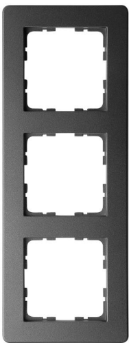
G1103B 3-gang W 86mm H 228mm D 9mm
