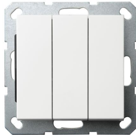
G3031 Three gang one way (1+1+1) 10AX 250V~
